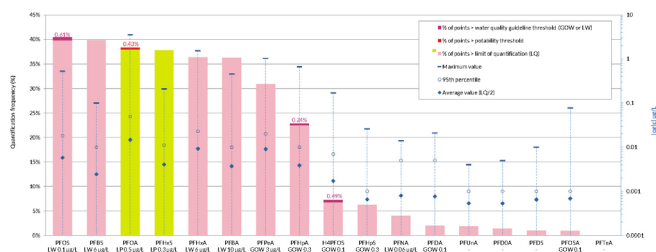
Figure 3: Per- and polyfluoroalkyl substances (PFASs) - Frequency of quantification and exceedance of German water quality guideline thresholds in Rhine groundwater (Gesundheitliche Orientierungswert or GOW, Leitwert or LW)
