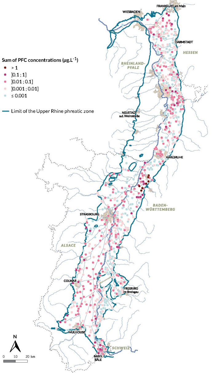
Figure 2. Map representing the sum of measured concentration of per- and polyfluoroalkyl substances (PFASs)
