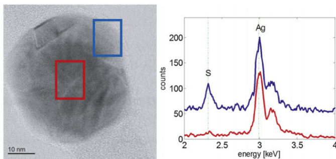
Figure 1: left: Transmission electron microscope (TEM) image of an Ag-NP reacted with wastewater. Energy dispersive X-ray (EDX) spectra of the red and the blue rectangles revealing different Ag/S ratios and thus different degrees of sulphidation are given on the right.
