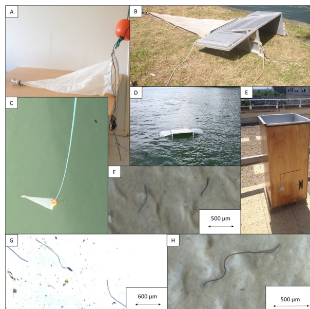
Figure 1: A/ Plankton net with a current meter that serves also as a ballast and a float that can be moved along the rope to fix the depth sampling. B/ Manta trawl. C/ Plankton net in deployment. D/ Manta trawl in deployment. E/ Atmospheric fallout collector. F, G and H/ Fibres encountered on different samples
