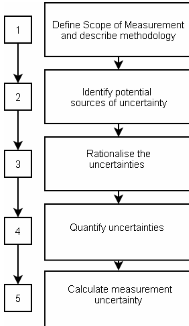
Figure 3 Steps to determine the measurement uncertainty
