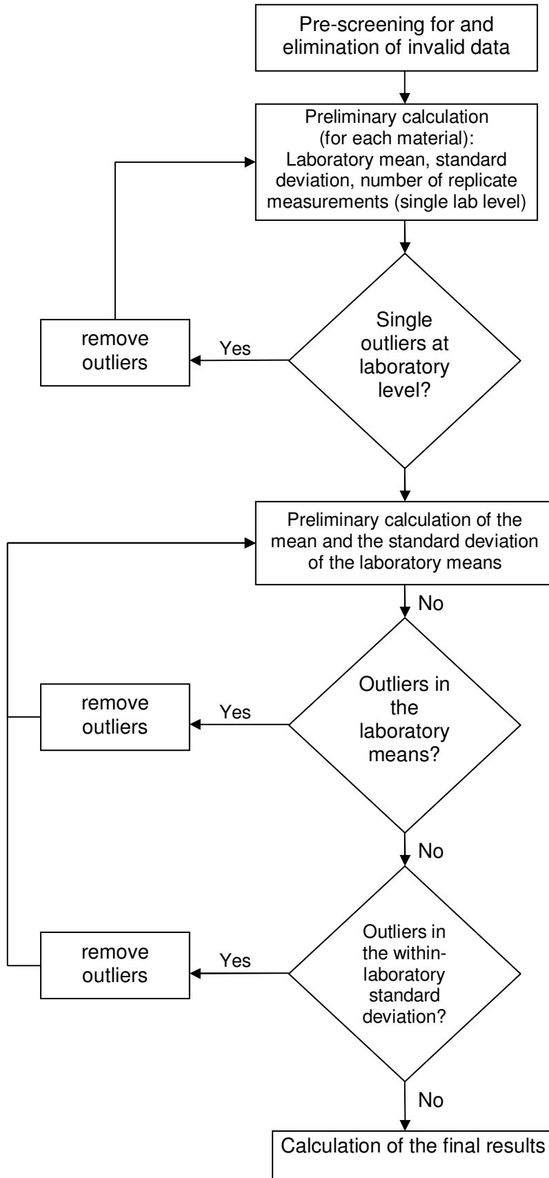
Figure 4 Flowchart of the main steps of the statistical analysis
